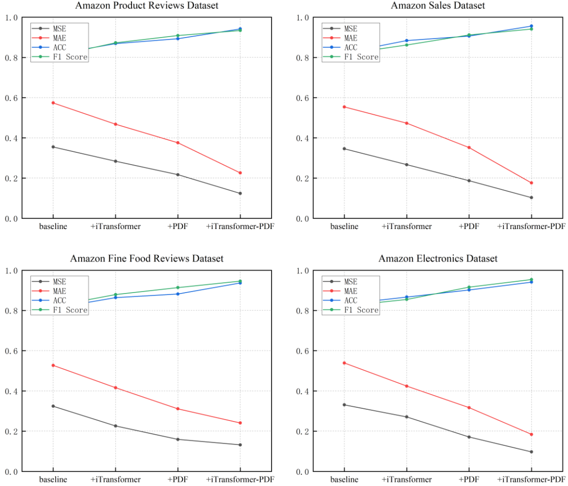
Figure 5. Visual Comparison of Ablation Experiments on Four Amazon Datasets
