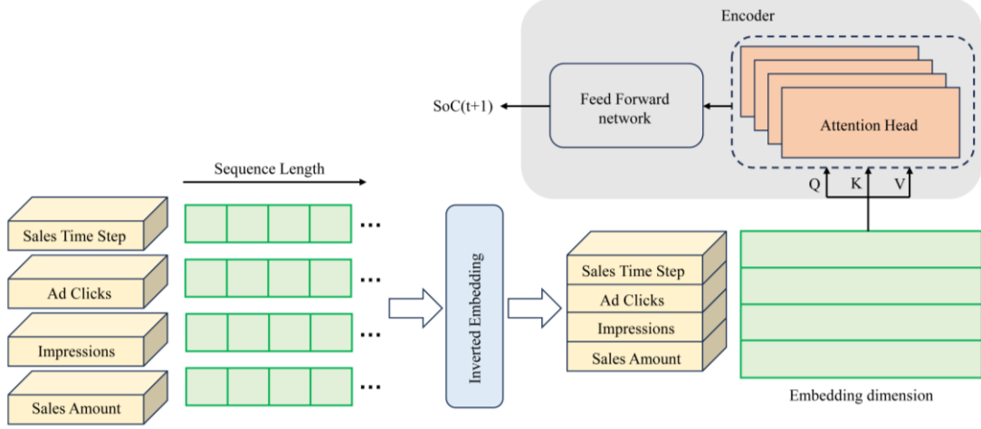
Figure 2. iTransformer model architecture diagram.
